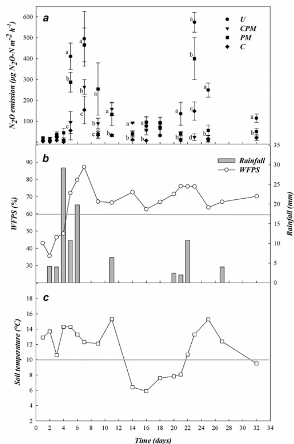
Figure 1. Evolution of a) the emission of N_2O in the Control (C, ♦) and after the application of Poultry Manure (PM, ■), Composted Poultry Manure (CPM, ▼) and Urea (U, ●); b) WFPS (- O -) and rainfall (■), and c) the soil temperature (- □ -). The horizontal line represents the water filled pore space (WFPS) value of 60% (b) and the corresponding temperature value of 10 ^{\circ}C (c). Different letters indicate significant differences between treatments for each measurement day.
