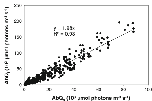
Fig. 4 Relationship between the absorbed quanta of C. fusca on filter ( AbQ_f ) and in suspension ( AbQ_s ) both expressed in \mu\text{mol photons m}^{-3} \text{s}^{-1} . The 11 irradiances supplied by the Junior-PAM were considered as well as samples from laboratory cultures under white light or from outdoor cultures grown under sunlight in a thin-layer cascade unit. The line shows the linear regression ( n=735 , p < 0.01 )
