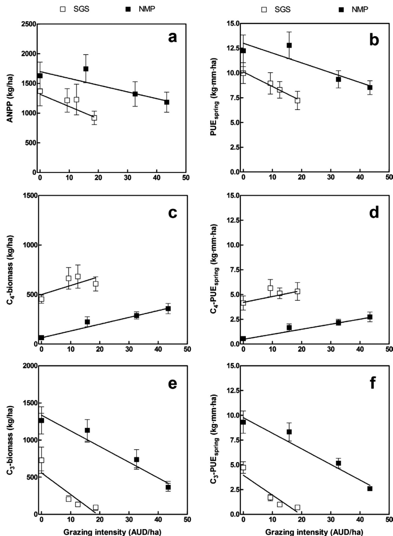
FIG. 2. Relationships between (a) aboveground net primary production (ANPP), (b) precipitation-use efficiency (PUE spring , ratio between ANPP and spring precipitation), (c) C 4 grass biomass, (d), C 4 -PUE spring (ratio between C 4 grass biomass and spring precipitation), (e) C 3 graminoid biomass, and (f) C 3 -PUE (ratio between C 3 graminoid biomass and spring precipitation) relative to grazing intensity (animal unit days, AUD/ha) for SGS and NMP. Points are mean values and error bars represent the 95% confidence intervals (CI). Lines represent the fitted values from linear mixed models.
