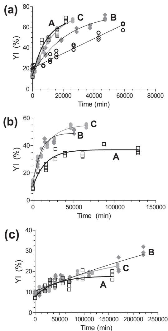
Fig. 2. Kinetics of browning development in alginate films stored at 25.0 °C and 75.2% (a), 57.7% (b) and 33.3% RH (c) [systems A (□), B (◆) and C (●)]. Zero-order kinetic of browning of a film developed by De'Nobili et al. (2013) with L-(+)-ascorbic acid and 109.6% of glycerol, without citric acid (75.2% RH, 25 °C) [(○)] (a).
