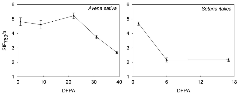
Fig. 4. Apparent fluorescence yield at 760 nm, SIF 760/a , for Avena sativa and Setaria italica under a PAR average intensity of 1000 \mu\text{mol m}^{-2} \text{s}^{-1} . DPAF means days after first panicle appeared. Error bars are SE (n = 10).
