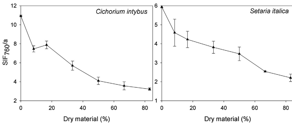
Fig. 5. Apparent fluorescence yield at 760, SIF 760/a , for Cichorium intybus and Setaria italica under a PAR average intensity of 1000 \mu\text{mol m}^{-2} \text{s}^{-1} . Error bars are SE (n = 5).
