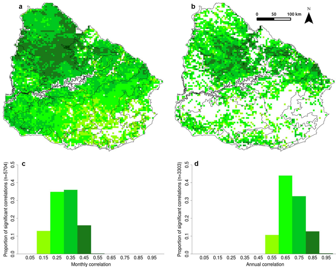
Fig. 6. Spatial (maps) and frequency (graphs) distribution of significant correlation between monthly fPAR values and monthly precipitation estimates from TRMM (a, c) and significant correlations between annual integral of fPAR and annual precipitation estimates from TRMM (b, d).
