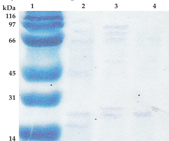
Fig. 2. SDS-PAGE of the purified PHBV depolymerase from Streptomyces sp. SSM 5670. Proteins were separated on a SDS-12% polyacrylamide gel and stained with Coomassie Brilliant Blue R-250. Lanes: 1, molecular weight marker ( \beta -galactosidase, 116 kDa; phosphorylase b, 97 kDa; serum albumin, 66 kDa; ovalbumin, 45 kDa; carbonic anhydrase, 31 kDa; lysozyme, 14 kDa); 2, concentrated culture supernatant; 3, concentrated DEAE Sephadex A-50 pool; 4, the purified PHBV depolymerase (arrow indicates location of protein).
