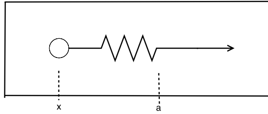
Fig. 1. A particle submitted to a spring, immersed in a heat bath.
