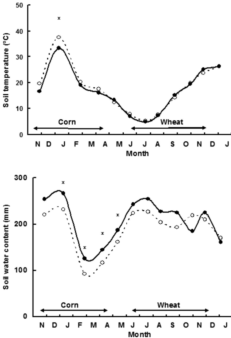
Figure 1. Soil temperature (0–10 cm) and water content (0–100 cm) during corn and wheat growing cycles under no till (●) and disk till (○).
