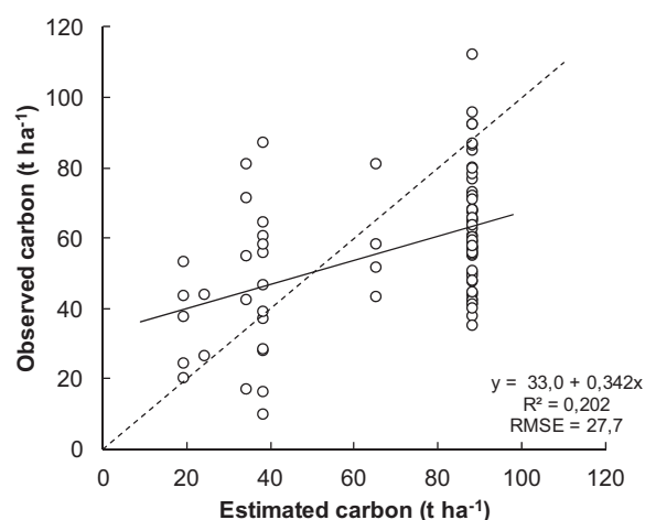
Fig. 2. Observed vs. estimated soil organic carbon (SOC) in the upper 30 cm of the profile using the IPCC Tool in uncropped fields of the Pampas. The estimated values correspond to the default values of SOC for native ecosystems and the observed SOC was measured in uncropped fields. The estimated regression intercept was greater than 0 and the slope lower than 1 ( P < 0.05 ).
