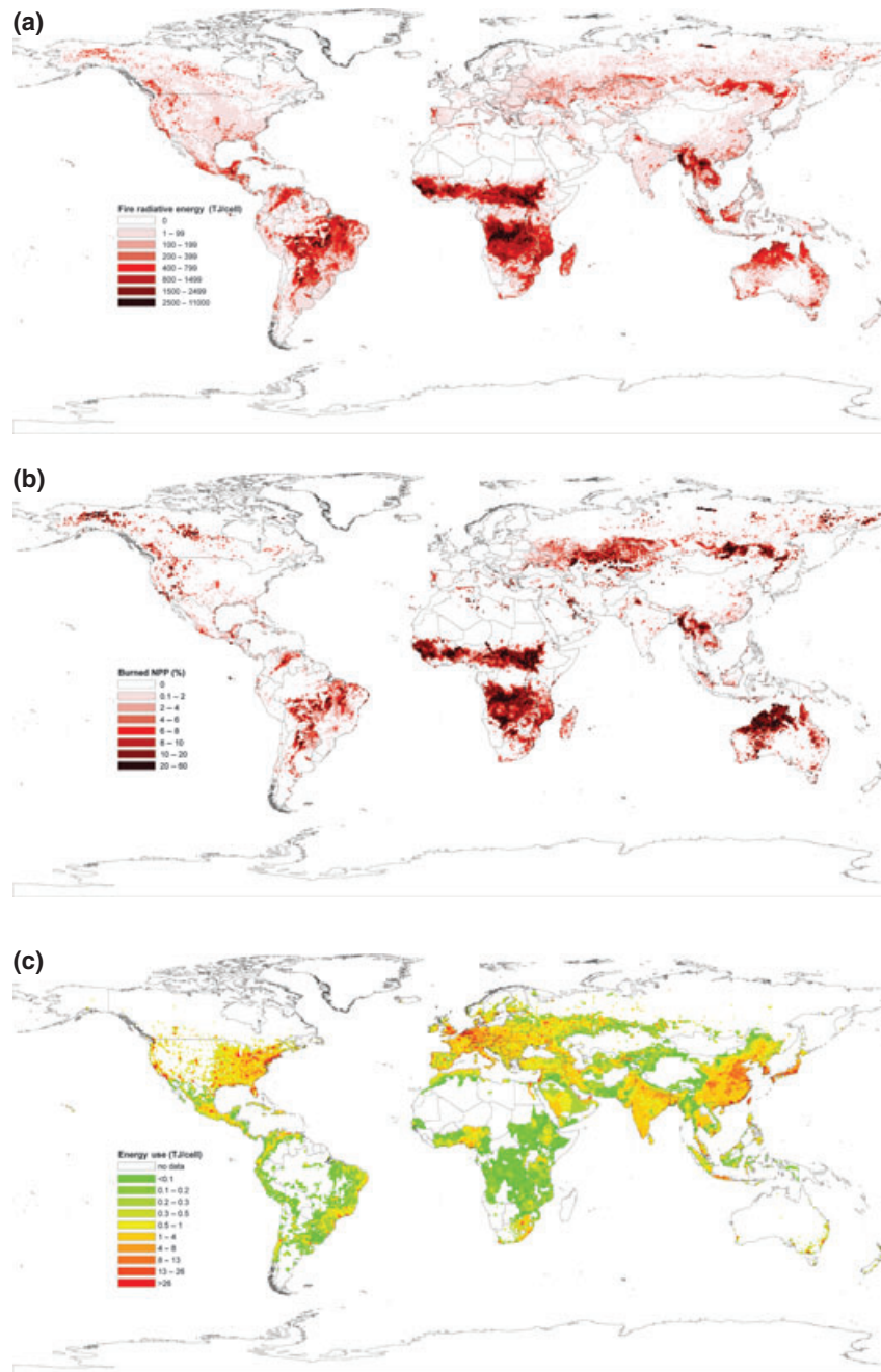
Fig. 1 Global distribution of wildfires and human energy consumption: (a) Radiative energy released by fires shown as the average energy flux ( \text{TJ yr}^{-1} ) per grid cell (0.5 by 0.5 degrees) estimated from the MOD14CMG product for the 2003–2010 period. (b) Percentage of mean net primary production (NPP) that burns in each grid cell to explain observed fire energy release rates (NPP values were obtained from the CASA model (Imhoff et al. , 2004)). (c) Energy use by humans ( \text{TJ yr}^{-1} ) per grid cell (0.5 by 0.5 degrees) based on the Gridded Population of the World (GPWv3) dataset and country-level estimates of per capita energy consumption from the International Energy Agency.
