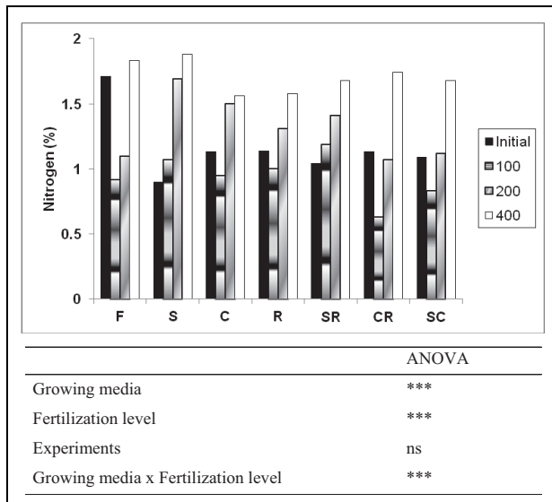
Fig. 3. Changes in nitrogen content (%) in the seven growing media tested fertilized weekly with 100 (A), 200 (B) or 400 (C) \text{mg L}^{-1} N related to the beginning of the experiment (initial). Data are mean of two replicates. Statistical significance: *** 0.001; ** 0.01; * 0.05; 'ns' not significant. Substrate abbreviations see Table 1.
