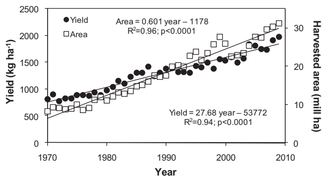
Fig. 1. Global world average yield (kg ha -1 ) and harvested area (million ha) of rapeseed for the period 1970–2009. Lines correspond to the adjusted linear regressions with the corresponding equations, correlation coefficients and probabilities.
