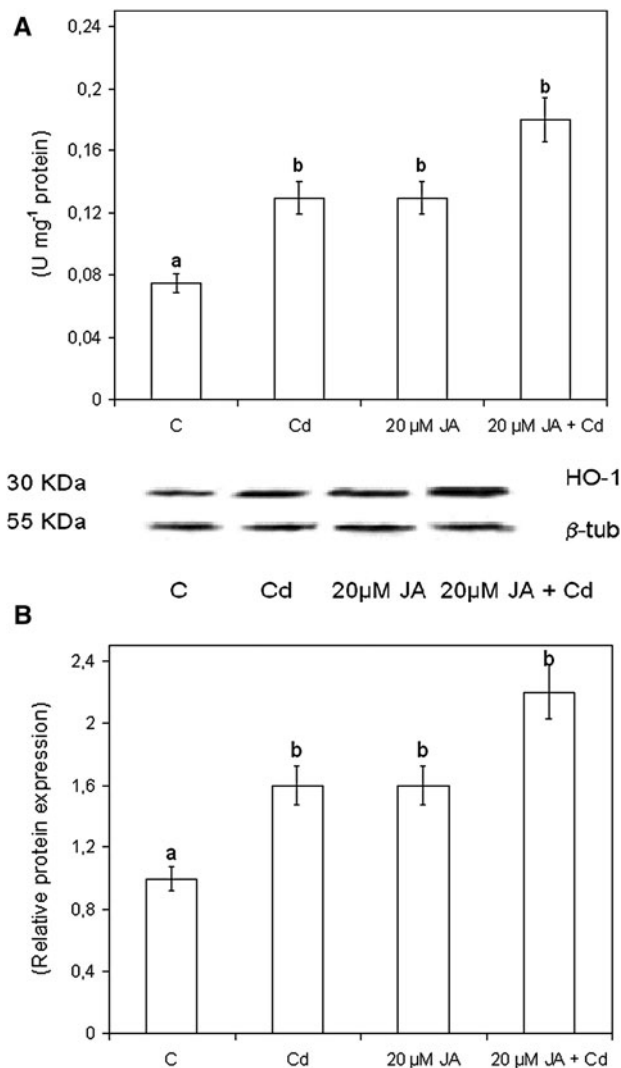
Fig. 5 Effect of Cd and JA pretreatment on HO activity ( a ) and amount of proteins ( b ) in soybean roots. HO-1 protein expression was analyzed by Western blotting as described in “Materials and Methods” Section. \beta -tubulin ( \beta -tub) immunoblotting was performed as an internal control of protein loading. Relative HO-1 protein expression taking control as 1 U. Experiments were performed as described in “Materials and Methods” Section. Values are the mean of three independent experiments and bars indicate SE. Different letters within columns indicate significant differences ( P < 0.05 ) according to Tukey’s multiple-range test
