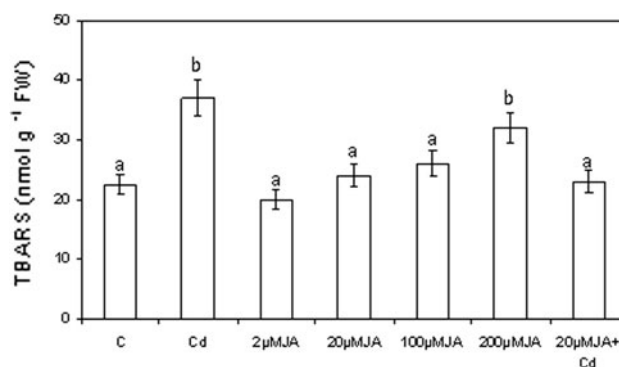
Fig. 2 Effect of Cd and JA pretreatment on TBARS formation in soybean roots. Experiments were performed as described in “Materials and Methods” Section. Values are the mean of three independent experiments and bars indicate SE. Different letters within columns indicate significant differences ( P < 0.05 ) according to Tukey’s multiple-range test
