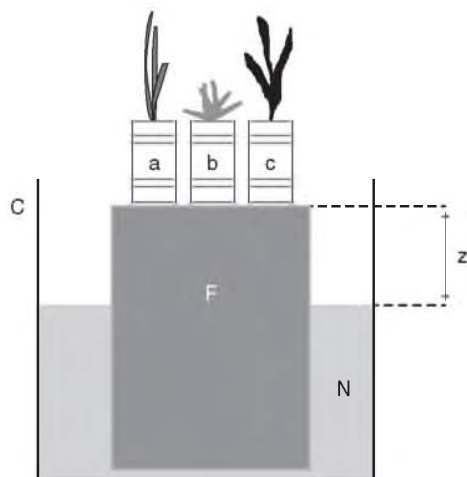
FIG. 1. Drought device, based on Snow and Tingey (1985). Abbreviations: C, plastic container; F, hygroscopic commercial foam; N, nutrient solution; a–c, sand-filled pots with a permeable base (polyester fabric); z, water-table depth (level of water stress). Redrawn from Fernández and Reynolds (2000).
