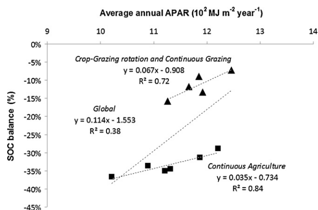
Fig. 6. Relationships between the average annual APAR (5 years) and SOC simulated balance (60 years under conventional tillage and no fertilization (SOC reference value (100%) = 79 t ha -1 )). Each point represents a crop sequence. Squares: Continuous agriculture; Triangles: Crop–rangeland rotation and continuous grazing.
