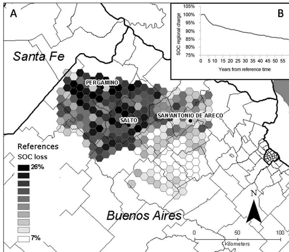
Fig. 7. (A) Simulated loss of SOC in 60 years, as % of the reference value ( 79 \text{ t ha}^{-1} ), in the Argiudolls of the Rolling Pampa. The value of each cell summarizes the effect of the observed management (crop sequence and tillage system with average fertilization). Santa Fe and Buenos Aires are provinces, Pergamino, Salto and San Antonio de Areco are towns and solid lines correspond to county limits. (B) Simulated loss of regional SOC, as % of the reference value, along 60 years.
