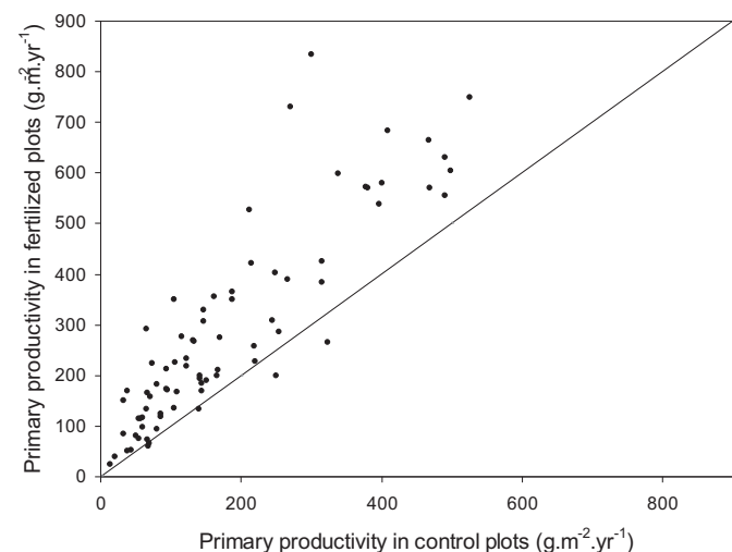
Fig. 2. The effect of N fertilization on aboveground net primary productivity in arid to subhumid ecosystems. Each data point represents a single comparison between fertilized and control treatments for a given field experiment ( n = 68 ). Values falling on the 1:1 line indicate no response to N fertilization treatment; points above the line indicate ANPP stimulation after N fertilization, whereas points below indicate lower ANPP in fertilized than control plots.
