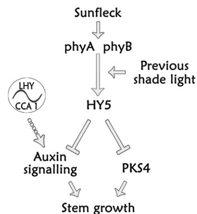
Figure 9. Model of the repression of shade-avoidance reactions by sunfleck induction of HY5 expression.
