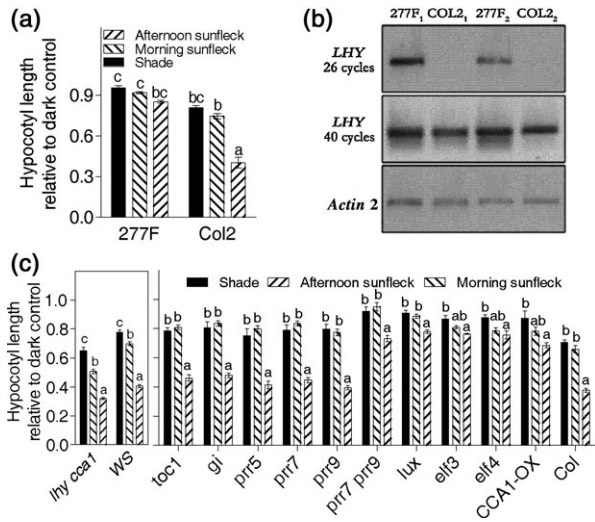
Figure 6. Dysfunction of the circadian clock impairs the response to sunflecks. (a) Hypocotyl length of the wild type (Col-2) and the 277F mutant grown under un-interrupted shade or shade interrupted daily by either a morning (at 0 h) or an afternoon (at 8 h) sunfleck. (b) Expression level of LHY determined by RT-PCR in 26 and 40 cycles in seedlings of the wild type and the 277F mutant. The expression level of ACTIN2 served as a control. (c) Hypocotyl length of the wild type (WS) and of the lhy cca1 mutant (left) or the WT (Col) and the toc1 , gi , prr5 , prr7 , prr9 , prp5 prr9 , lux , elf3 and elf4 mutants, and the transgenics overexpressing CCA1 (right) grown under the conditions described in (a). Interactions: P = 0.0004 (a); P < 0.003 (c). Data are means and SEs of between three and eight replicate boxes. Different letters denote significant differences ( P < 0.05 ) among means of each genotype.
