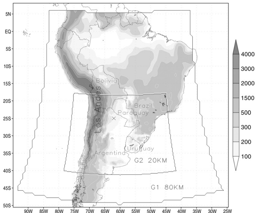
Fig. 2. Nested domains over South America and adjacent oceans. Topography is shaded and indicated in meters. A cross indicates the location of the vertical profile in Fig. 3.
