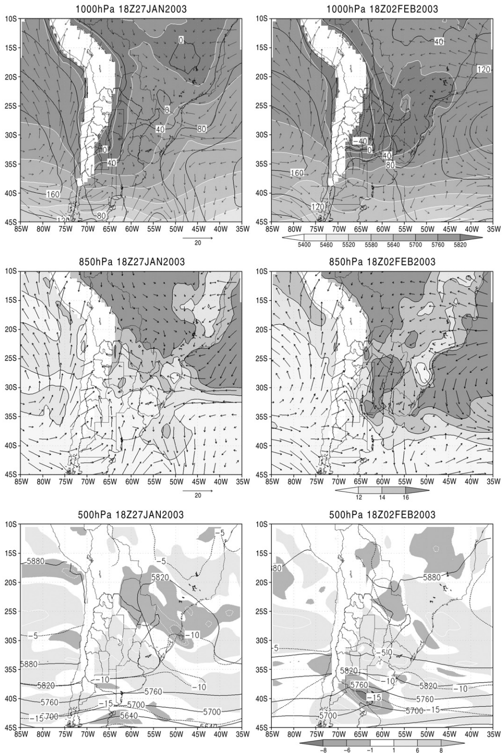
Fig. 4. Upper panels: 1000/500 hPa thickness (dmgp)(shaded), 1000 hPa geopotential height (mgn)(contours) and wind vector (m/s)(arrows). Center panels: 850 hPa wind vectors (m/s)(vectors) and mixing ratio (g/kg)(shaded). Lower panels: 500 hPa geopotential (mgn)(contours) and relative vorticity ( 1/s \cdot 10^5 ) (shaded). Left panels for January 27, Right panels for February 2nd, both at 18 UTC.
