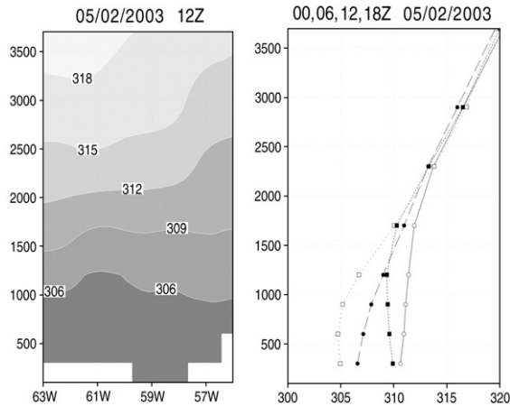
Fig. 3. Virtual potential temperature ( ^{\circ}\text{K} ) for February 5. Left: vertical cross section at 25^{\circ}\text{S} at 12 UTC. Right: vertical profiles at 25^{\circ}\text{S} 62^{\circ}\text{W} at 00 (solid line), 06 (long dash), 12 (dotted) and 18 (short dash) UTC. The altitude is indicated in meters.
