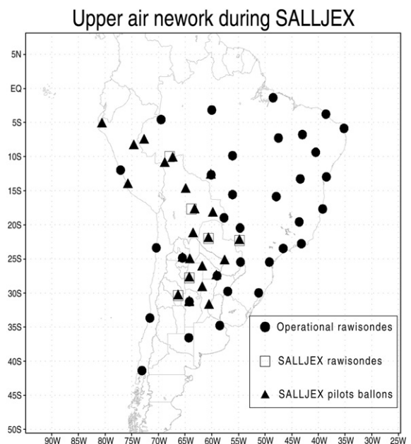
Fig. 1. Spatial distribution of upper air observations during SALLJEX.
