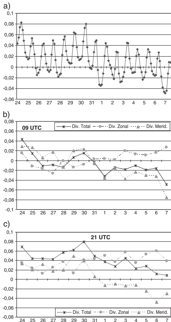
Fig. 12. Boundary layer divergence ( 1/s \cdot 10^4 ) averaged over the domain shown in Fig. 5. a) Total divergence from 24 January at 09 UTC to 7 February at 21 UTC every 3 hours. b) and c) Total, zonal and meridional divergence at 9 UTC and at 21 UTC, respectively.
