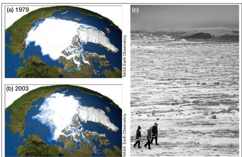
Figure 5. Satellite images of the areal extent of summer Arctic sea ice from (a) 1979 to (b) 2003. The coverage of sea ice in the summer has declined markedly. (c) Researchers study the fragile Arctic landscape in Thule, Greenland, where global change is likely to have the strongest effects on communities and ecosystems.
