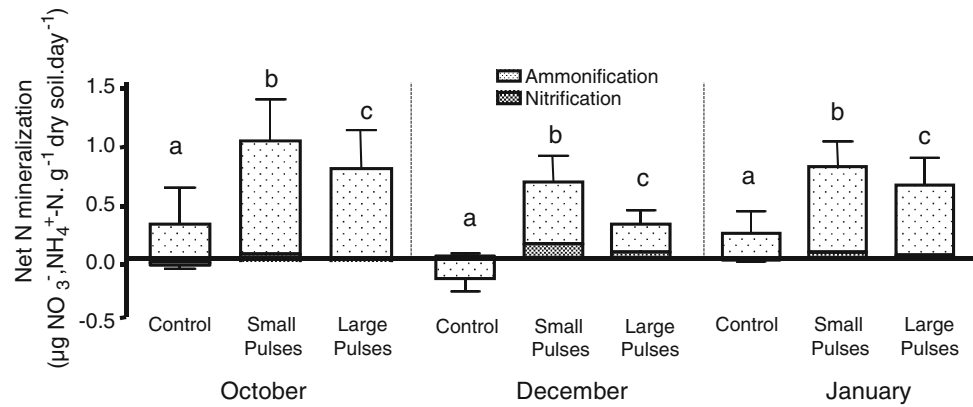
Figure 2. Net nitrification, net ammonification, and net nitrogen mineralization in irrigation treatments and control at 0–10 cm depth, measured in situ during 5-day periods when manipulations were applied. Bars represent mean values (+SE) for n = 20 . Different letters show significant differences among treatments within each date at P < 0.10 .
