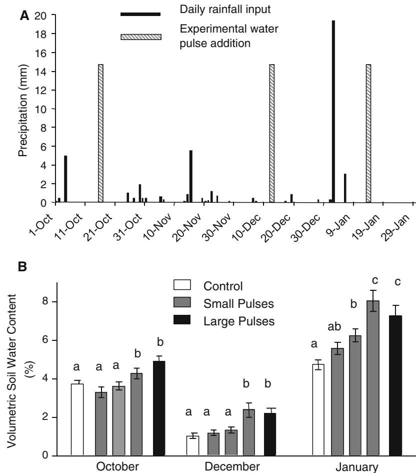
Figure 1. Effects of water-manipulation treatments on rainfall inputs ( upper panel ) and volumetric soil water content at 0–20 cm depth ( lower panel ) for the studied growing season October–January. A Daily rainfall inputs: thin bars correspond to rainfall events at the study site; dashed bars correspond to water irrigation in plots from the pulse treatments that received 15 mm experimental events, in October, December and January, in three small or one large-pulse event in each occasion. B Volumetric soil water content: open bars correspond to treatments receiving ambient rainfall quantities ( control ) and solid bars correspond to treatments with small ( gray ) or large ( black ) irrigation pulses, measured after pulse addition; bars represent mean values ( \pm SE) with n = 20 . Different letters show significant differences among treatments within each date at P < 0.05 .
