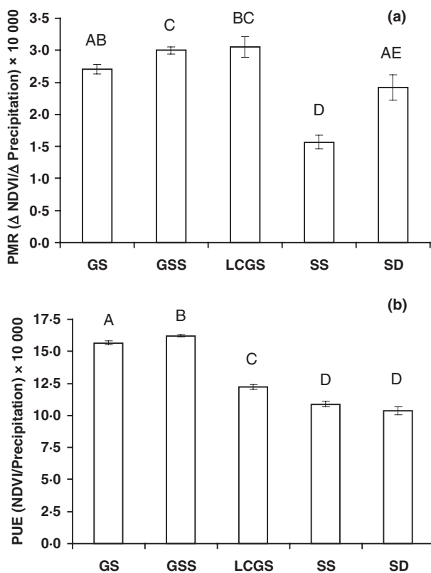
Fig. 4. PMR (a) and PUE (b) per physiognomic class. Bars indicate mean \pm spatial standard error. GS: grass steppes, GSS: grass-shrub steppes, LCGS: low cover grass steppes, SS: shrub steppes and SD: semi-deserts. PMR and PUE values were multiplied by 10 000. Capital letters indicate significant differences ( P < 0.05 ) according to the linear mixed model applied.
