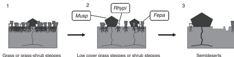
Fig. 1. State and transition scheme for the Festuca pallescens grasslands of the Sub-Andean district. Numbers refer to increasing degradation states. Musp stands for the deciduous shrub Mulinum spinosum , Rhypi for the mesophytic perennial grass Rhytidosperra picta and Fepa for the perennial grass Festuca pallescens . Adapted from Paruelo (2005).
