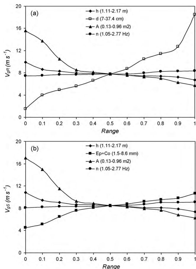
Fig. 6. Sensitivity analysis for model variables. Variations in root ( V_{gr} ) (a) or stem ( V_{gs} ) (b) failure wind speed ( \text{m s}^{-1} ) in response to changes in the values of model variables between 0 (minimum) and 1 (maximum). h : plant height; d : root plate diameter; Ep + Co : thickness of epidermis plus cortex; A : area expected to be loaded by wind gusts; n : natural frequency. Calculations were performed at decile intervals across the full observed range (indicated in brackets next to symbol codes) for each variable and are centred on the observed mean value (i.e., 0.5) for each variable.
