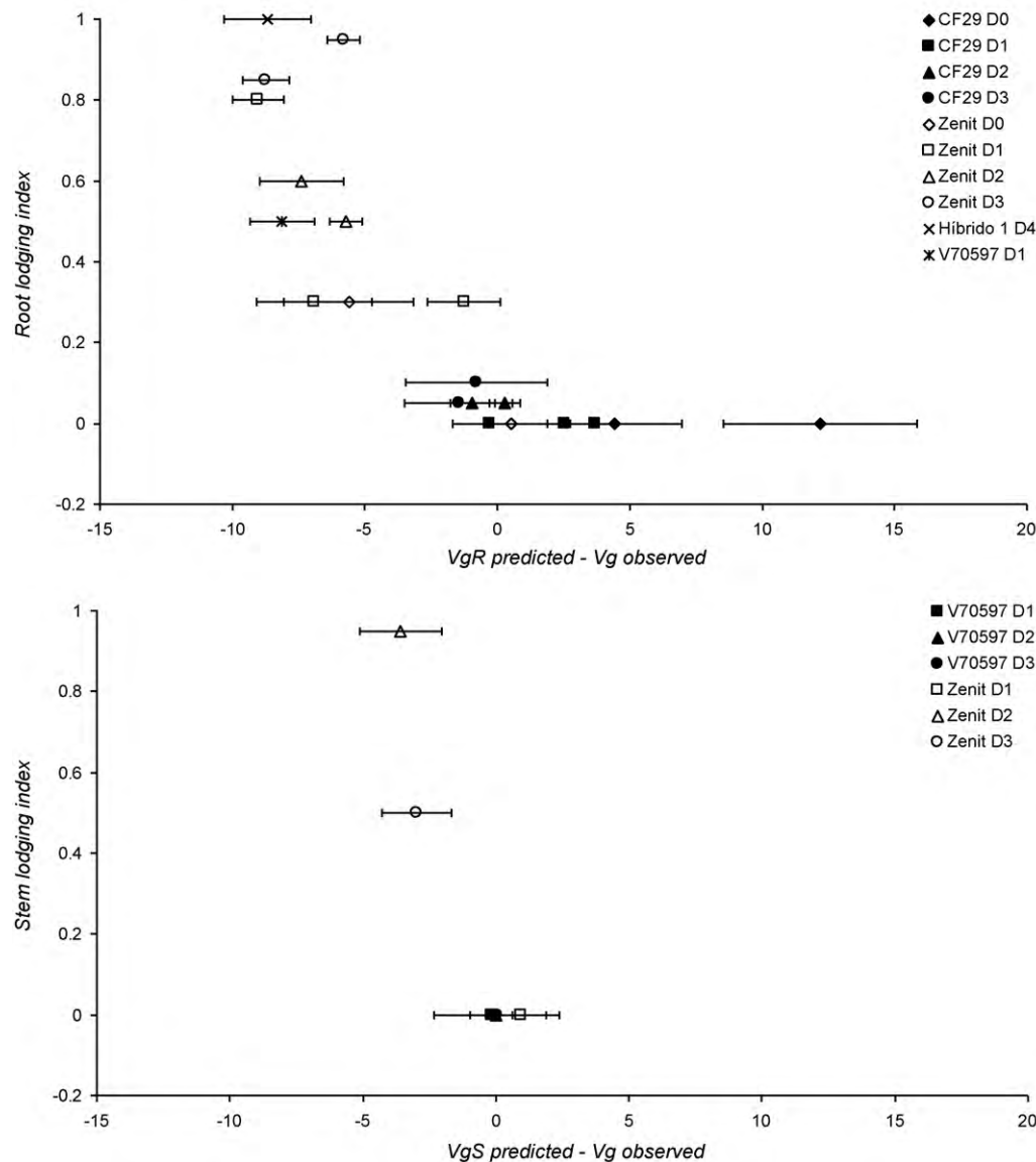
Fig. 5. Relationship between root (a) or stem (b) lodging index and the difference between predicted and observed root ( VgR ) or stem ( VgS ) failure wind speed for each lodging event. D0: 3 plants m^{-2} ; D1: 5.6 plants m^{-2} ; D2: 10 plants m^{-2} ; D3: 16 plants m^{-2} . Horizontal bars indicate \pm 1 standard deviation ( n = 10 ).
