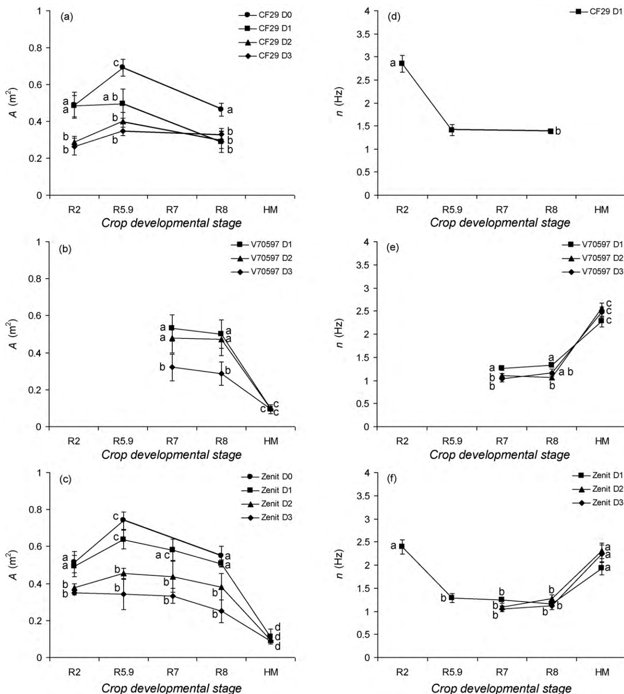
Fig. 2. Area loaded by wind gusts ( A , \text{m}^2 ) (a–c) and plant natural frequency ( n , Hz) (d–f) for CF29, V70597 and Zenit, between R2 and harvest maturity (HM) for plants growing at four plant densities, D0: 3 plants \text{m}^{-2} ; D1: 5.6 plants \text{m}^{-2} ; D2: 10 plants \text{m}^{-2} ; D3: 16 plants \text{m}^{-2} . Three experiments were used for panels a (E1, E2 and E3 from Sposaro et al., 2008) and b (E1, E2 and E3 from Hall et al., 2010); six experiments were used for panel c (from Sposaro et al., 2008 and Hall et al., 2010); Two experiments were used for panels a (E1 and E2 from Sposaro et al., 2008) and b (E1 and E2 from Hall et al., 2010); four experiments were used for panel c (first two seasons from Sposaro et al., 2008 and Hall et al., 2010). Error bars indicate \pm one standard error (with 3 replicates). Different letters next to symbols indicate significant ( p < 0.05 ) differences across crop population densities and developmental stages for each hybrid.
