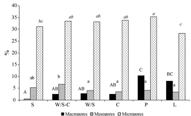
Fig. 3. Average pore-size distribution of 0–0.04 m layer. Different letters indicate significant differences between treatments for each category of pores ( p < 0.05 ).
