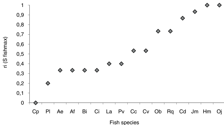
Figure 4. Relative rank of S_{fishmax} ( r_i = (S_{fishmax_i} - 1)/(n - 1) ), where r_i is the relative rank of the i th species, S_{fishmax_i} is the value of the Secchi disc depth that gave rise to the largest abundance of the i th species and n is the number of observations) for the 16 species collected in the upper Salado River lakes. Species codes as in Table 2.
