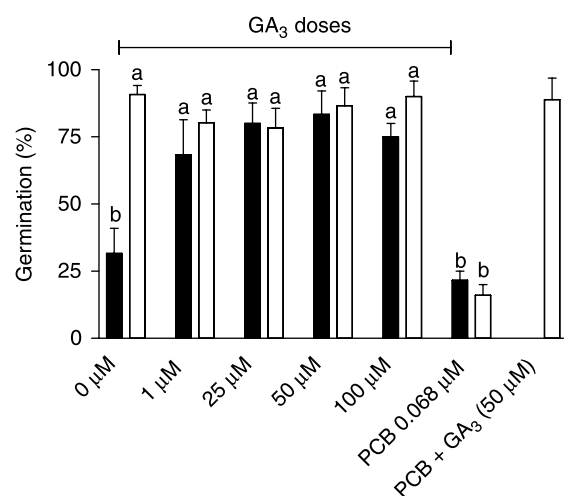
Figure 4. Final germination percentages of Cynara cardunculus seeds incubated at fluctuating temperatures (25/15°C) (open bars) or at a constant temperature (20°C) (filled bars) incubated in different solutions (see legend beneath horizontal axis). Vertical bars indicate the SEs. Germination experiments were performed for 14 d. Different letters at the top of each bar indicate significant differences according Tukey's test ( \alpha = 0.05 ).
