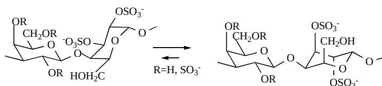
Fig. (7). Sulfated galactan from Gelidium crinale . Conformational equilibrium of the 4-linked 2,3-disulfated α-L-galactose units.
