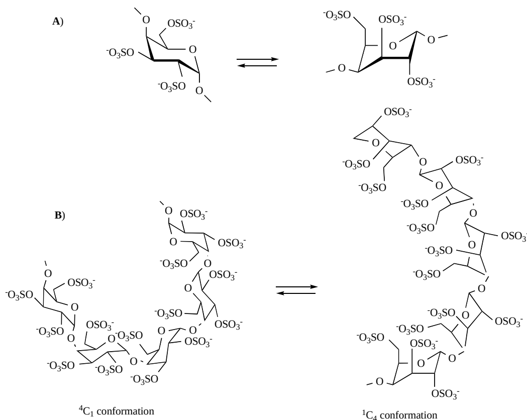
Fig. (1). A) Equilibrium between ^4\text{C}_1 and ^1\text{C}_4 chair conformations of an oversulfated (1 \rightarrow 4)- \alpha -D-galactose unit in a galactan backbone. B) Change in the galactan backbone shape with the inversion of the configuration of the pyranose cycle of the sugar unit.
