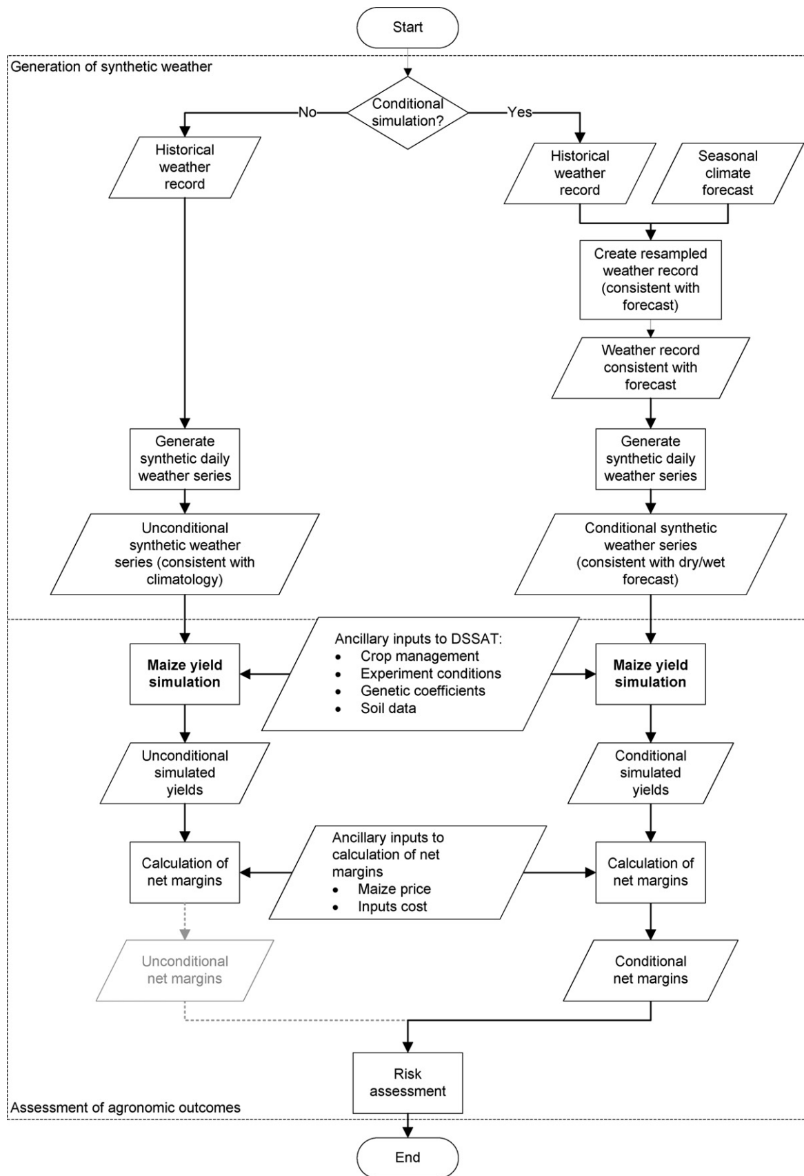
Fig. 1. Schematic diagram of the coupled SWG generator and DSSAT cropping system model.
