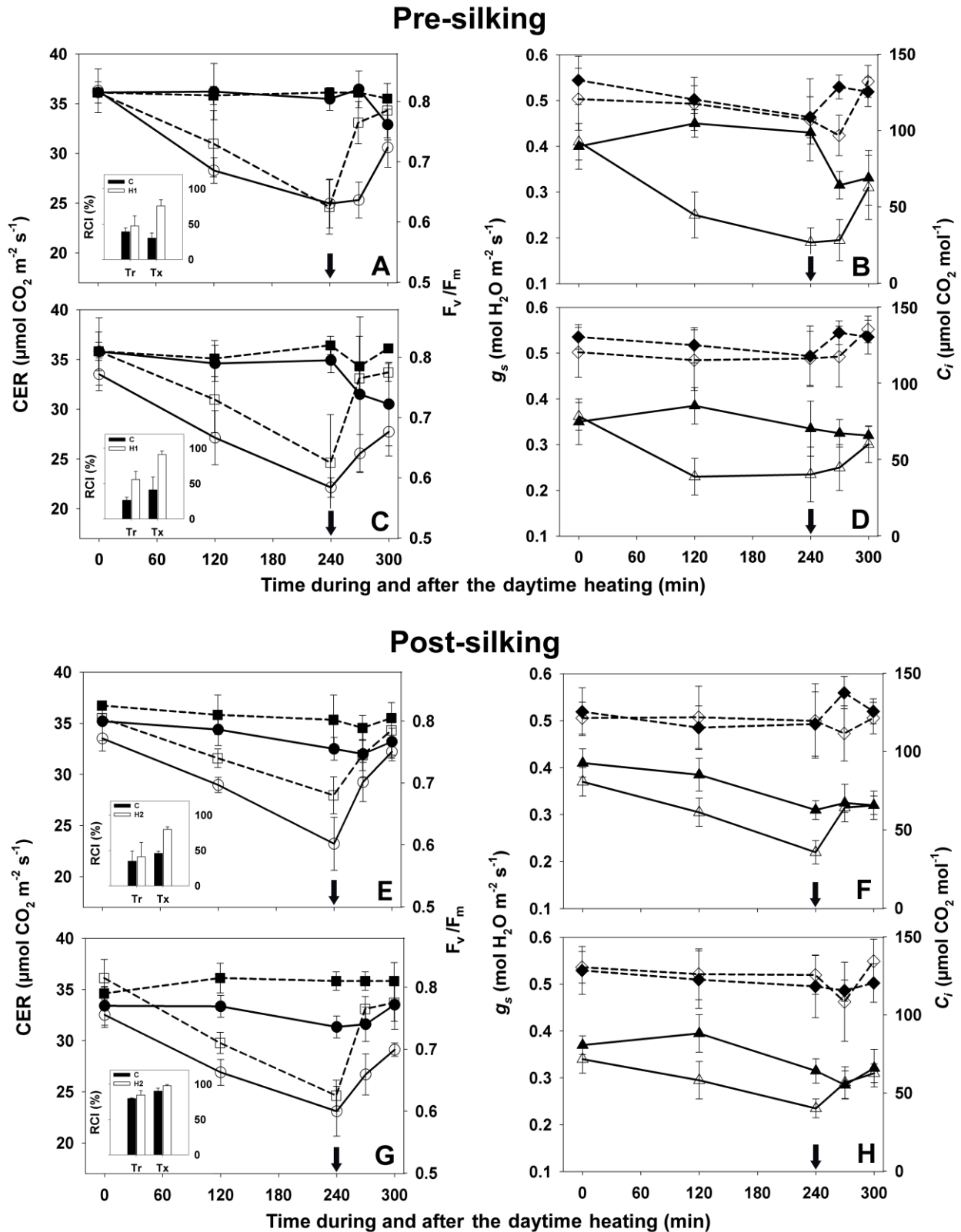
Fig 1. Leaf photosynthesis rate (CER, circles), maximum efficiency of PSII ( F_v/F_m , squares), stomatal conductance ( g_s , triangles) and internal CO_2 concentration ( C_i , diamonds) as a function of time during and after the daytime heating. Data corresponds to the average of two maize cultivars under control (closed symbols) and heat conditions (open symbols). Arrows indicate the time when shelters were reopened at the end of the daytime heating treatment. Measurements were taken on day 7 (A, B, E and F) and day 14 (C, D, G and H) after the start of the heating period in pre- and post-silking. Relative cell injury (RCI) was also measured (inset) 120 min after initiating the daytime heating in both cultivars (Tr: tropical and Tx: tropical \times temperate). Leaf photosynthesis data (CER) were partially obtained from Neiff et al., 2016.
