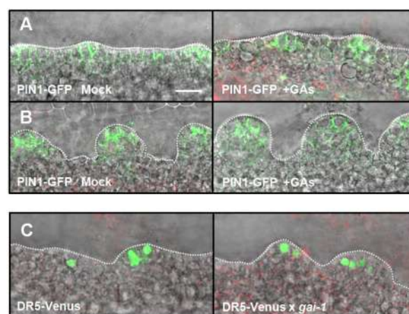
Fig. 5. GAs do not alter auxin transport or response in ovule primordia. (A,B) Ovule primordia of the pPIN1:PIN1-GFP line upon GA treatment, at stage 1-I (A) or 1-II (B) of ovule development. (C) Ovule primordia at early stage 1-II of pDR5:3xVENUS and pDR5:3xVENUS lines crossed with gai-1 mutant. Scale bars: 10 µm.
