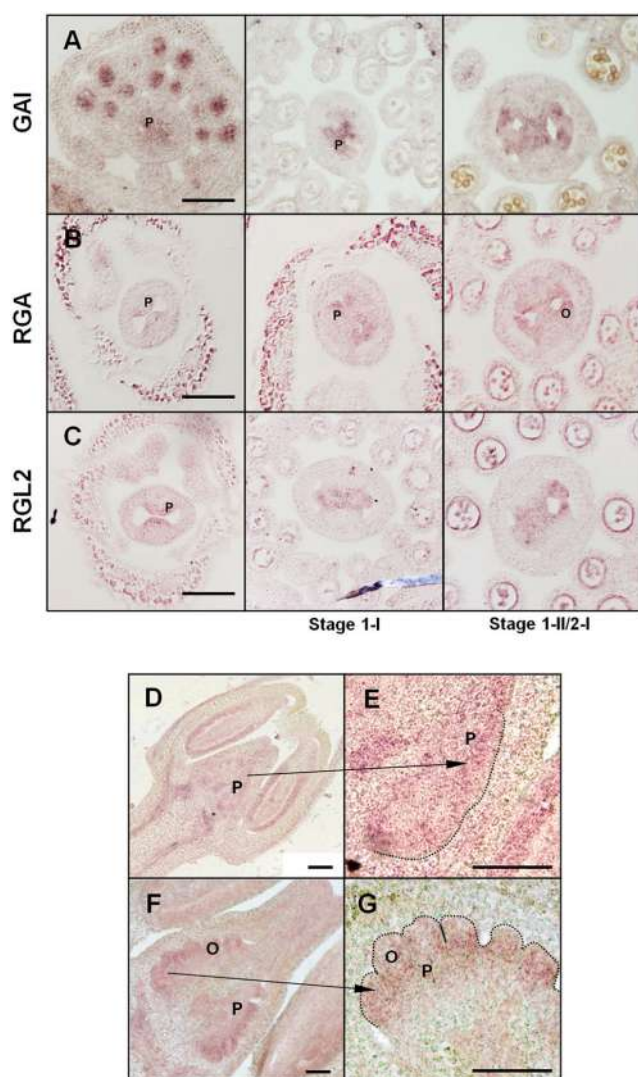
Fig. 4. DELLA genes are expressed in placental tissue. (A-C) Expression of GAI, RGA and RGL2 in placenta and ovule primordia. In situ mRNA hybridization was used to detect transcripts of GAI (A), RGA (B) and RGL2 (C). Pistils at the developmental stage before ovule primordia initiation (left panels), ovules at stage 1-I (central panels), and ovules at stage 1-II/2-I (right panels). (D-G) In situ mRNA hybridization of PROCERA in tomato ovaries during early developmental stages. Scale bars: 100 µm. O, ovule primordium; P, placenta.
