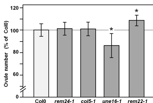
Fig. 6. Null mutants of UNE16 and REM22 show altered ovule number.
