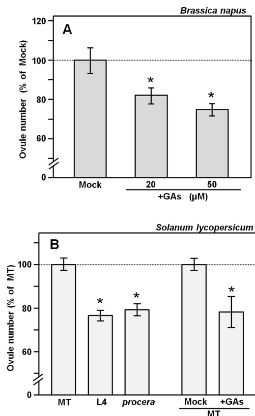
Fig. 3. GAs also regulate ovule number in rapeseed and tomato. (A) Ovule number in mock- and GA-treated rapeseed ( Brassica napus L.) Topaz DH4079. GAs were applied by watering plants with 2 \times 10^{-5} and 5 \times 10^{-5} M GA_4+GA_7 . More than 20 pistils were used, and experiments were repeated twice, with similar results. (B) Ovule number in tomato MT ( Solanum lycopersicum L.), in the L4 line overexpressing a GA20ox1 gene, in the procera mutant, and in GA-treated ( 10^{-5} M) MT plants. Ovule number in tomato was determined from at least six ovaries, and the experiment was repeated three times, with similar results. Data represents mean±s.d. Significant differences (Student's t -test) with the WT/mock are indicated by an asterisk (* P <0.01). Values were normalized to the corresponding WT or mock plants.
