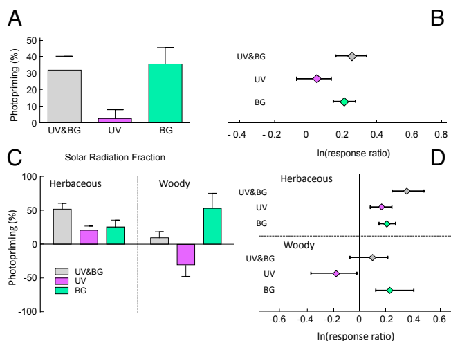
Fig. 2. Exposure to solar radiation facilitates subsequent microbial decomposition. (A) Enhancement of microbial decomposition (photopriming) in a 45-d field soil incubation, evaluating the wavelength-dependent effects of prior exposure to solar radiation. Photopriming is defined as the percent increase for each species in biotic decomposition due to exposure to different wavelengths of solar radiation. Wavelength effects are calculated as indicated in Fig. 1. Each bar represents the average of 23 species (+1 SEM). (B) Mean effect sizes of the different wavelengths on photopriming across the 23 species ( \pm 95\% CI). Details of metaanalysis can be found in Table S3. (C) Photopriming effects on decomposition, partitioned for herbaceous and woody species. Each bar represents the average of the group ( n = 13 for herbaceous species; n = 10 for woody species, +1 SEM). (D) Mean effect sizes of solar radiation on photopriming, partitioned by herbaceous and woody species. Litter quality analyses and analysis of grouping for herbaceous and woody species can be found in Table S2 and Fig. S1.
