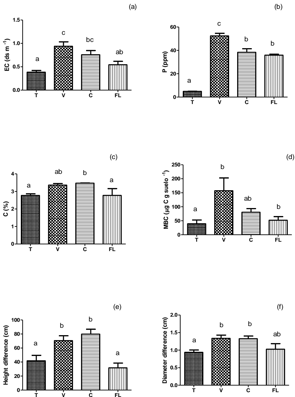
Figure 1. Mean values of (a) soil electrical conductivity (EC), (b) exchangeable phosphorous (P), (c) oxidable carbon (C), (d) microbial biomass carbon (MBC), (e) differences in plant height and (f) differences in plant diameter between two consecutive years.
